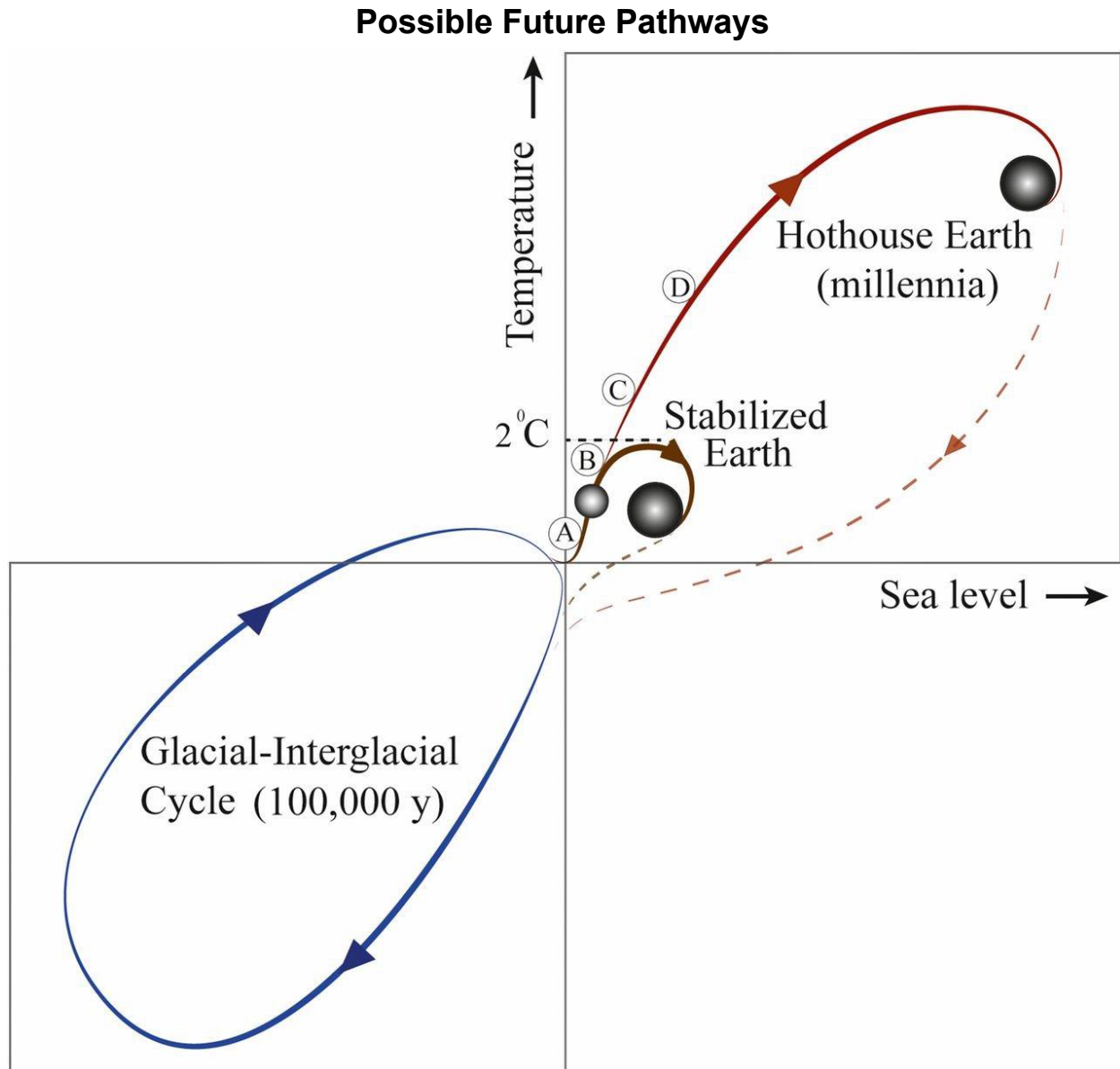
Figure 8. Possible Future Pathways
