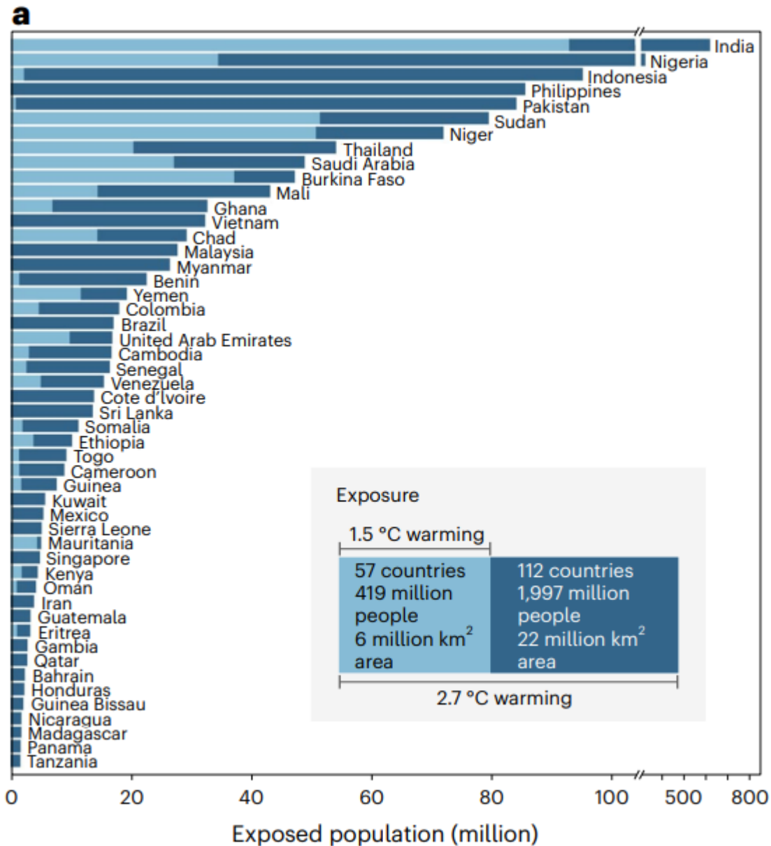
Figure 20. Country-level Exposure to Unprecedented Heat
