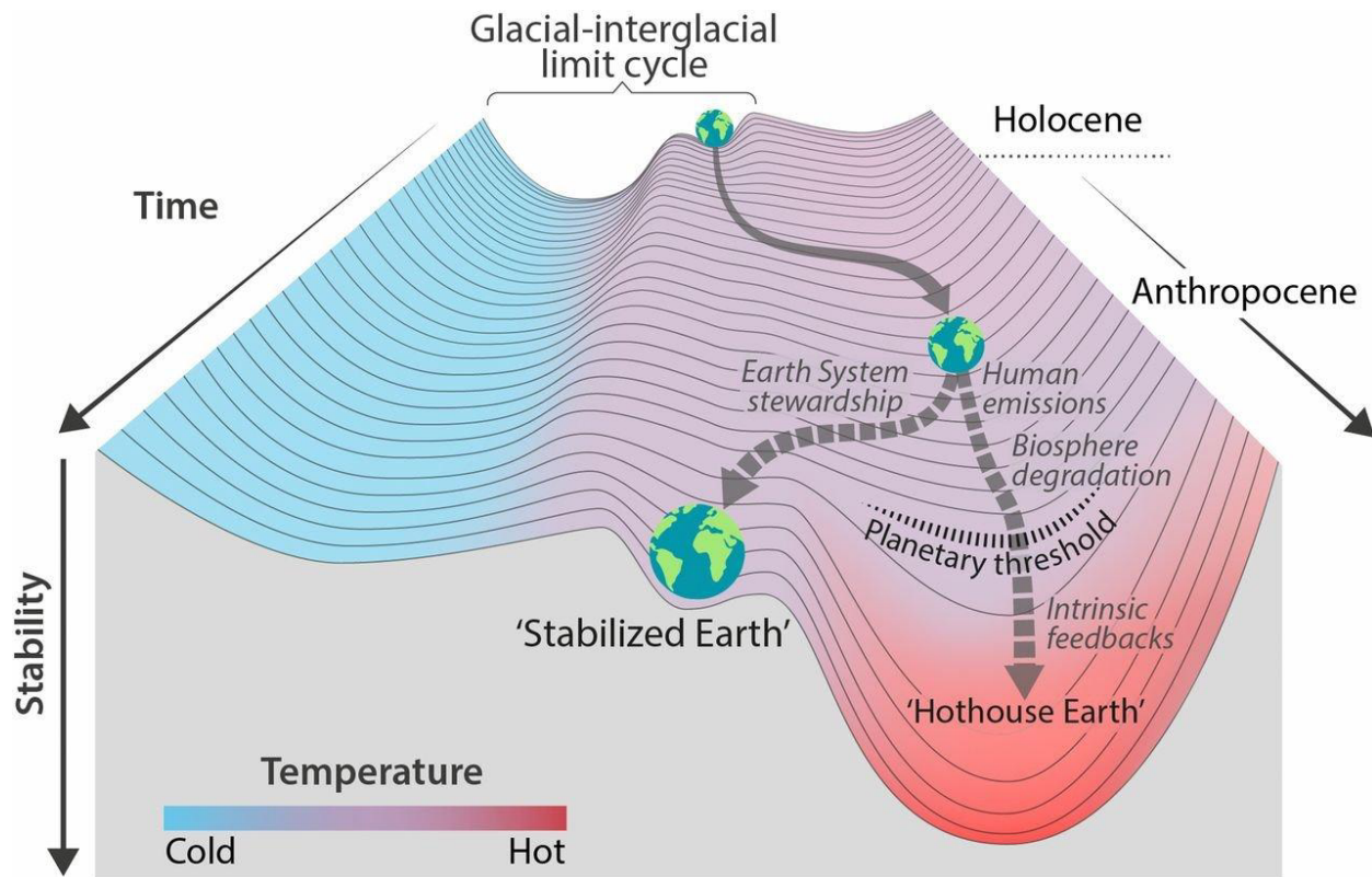
Figure 9. Pathways of the Earth System Out of the Holocene
