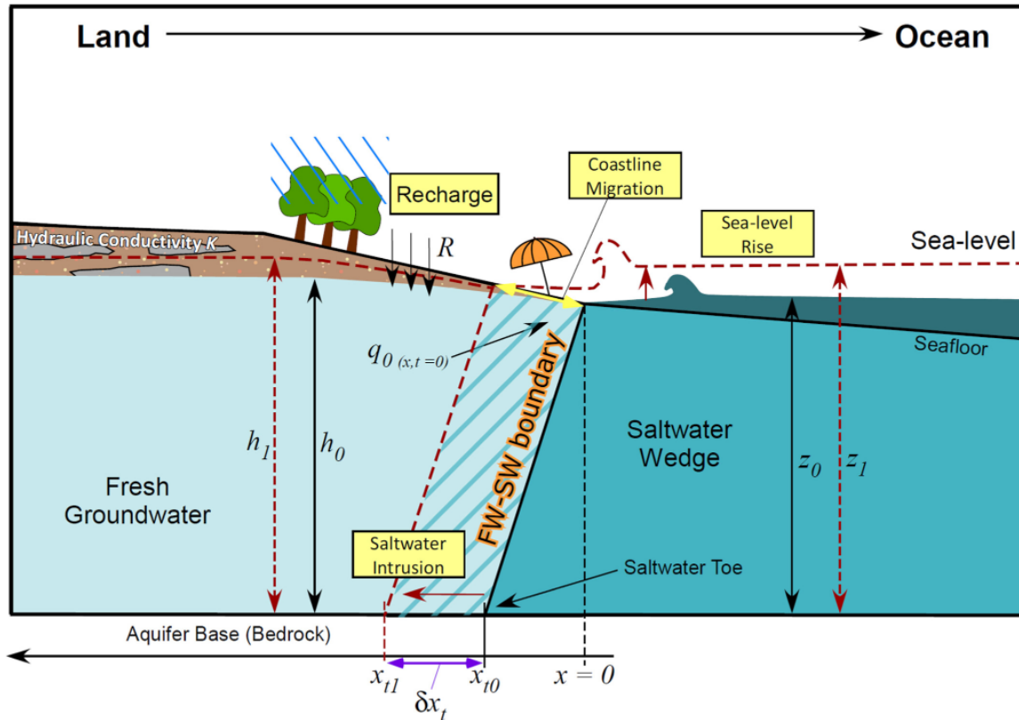
Figure 5. A Coastal Aquifer Undergoing Saltwater Intrusion
