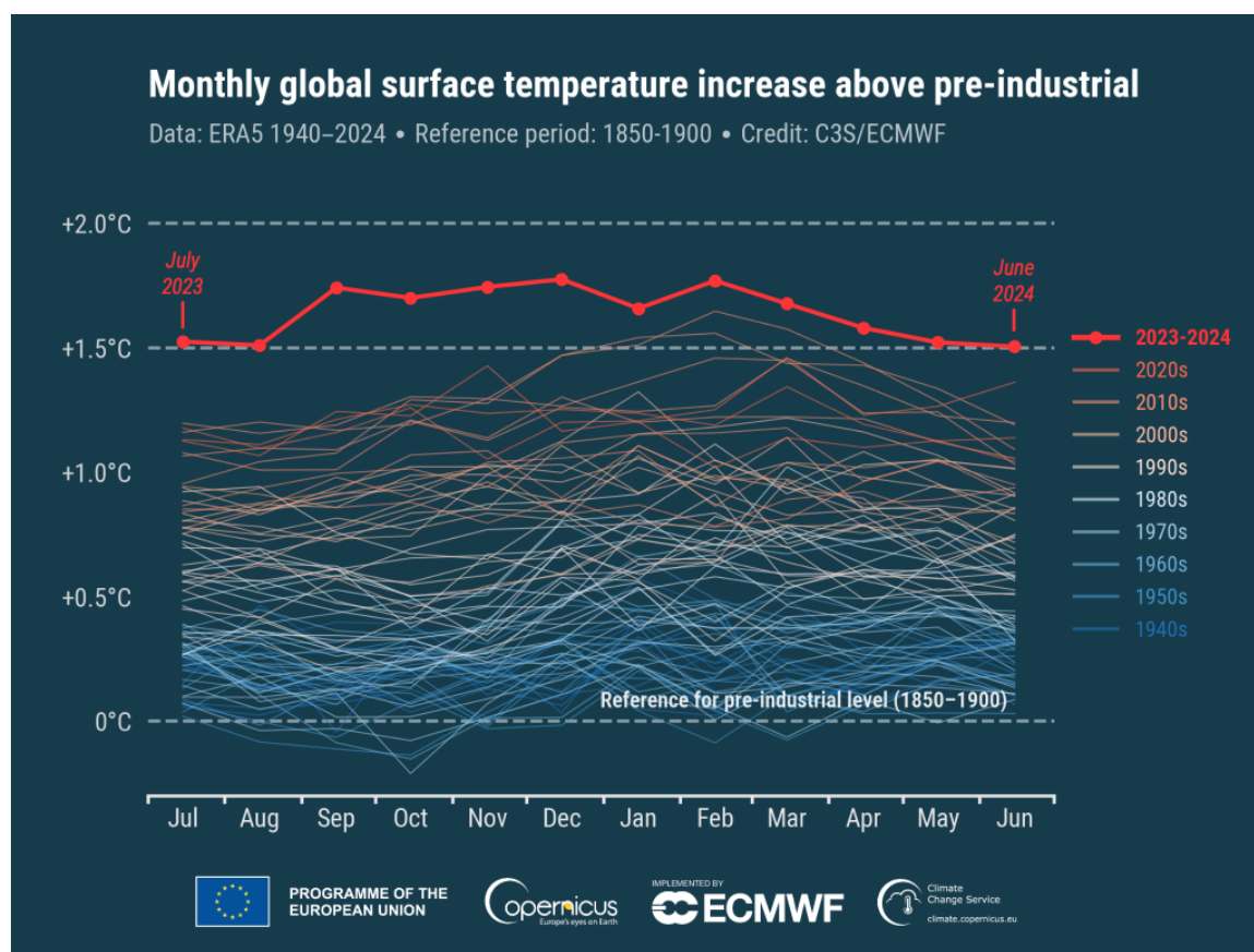
Figure 14. Monthly Global Surface Air Temperature Increases Above Pre-industrial Levels
