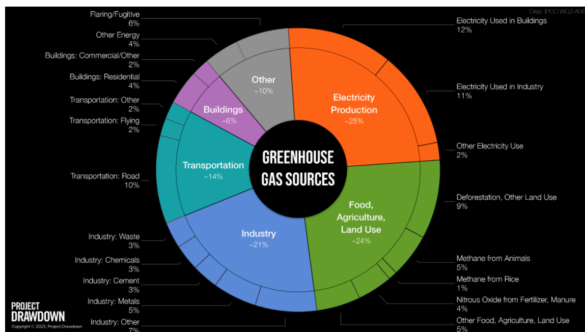
Figure 25. Greenhouse Gas Sources by Sector
