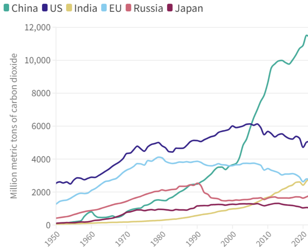
Figure 7. Annual Emissions from Fossil Fuels and Industry 59
