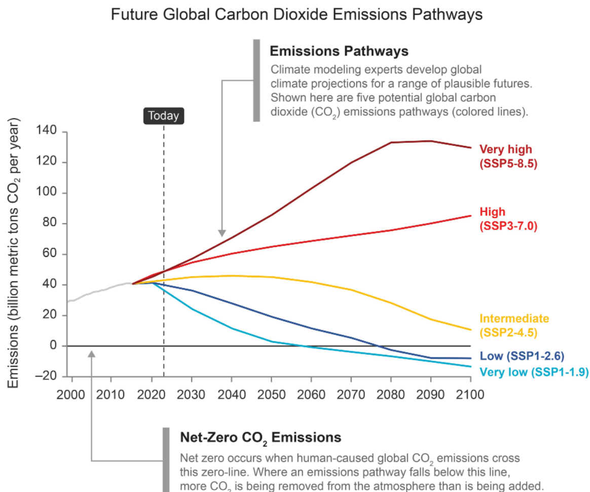
Figure 22. Future Global Carbon Dioxide Emission Pathways
