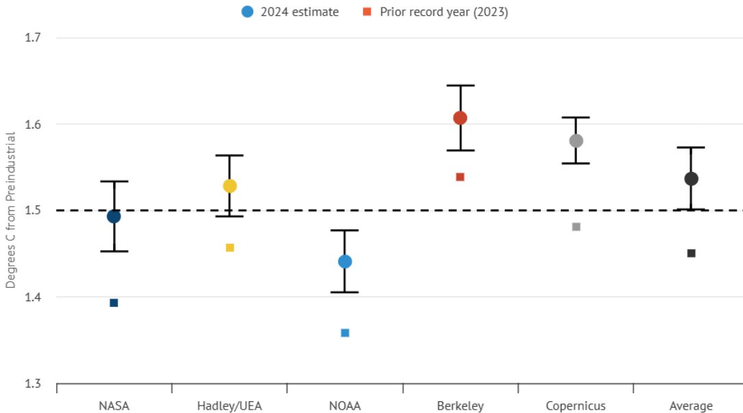
Figure 15. Estimates of 2024 Temperatures
