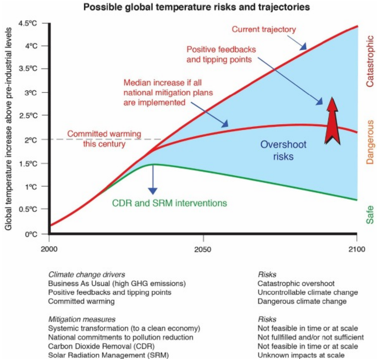
Figure 10. Possible Global Temperature Risks and Trajectories
