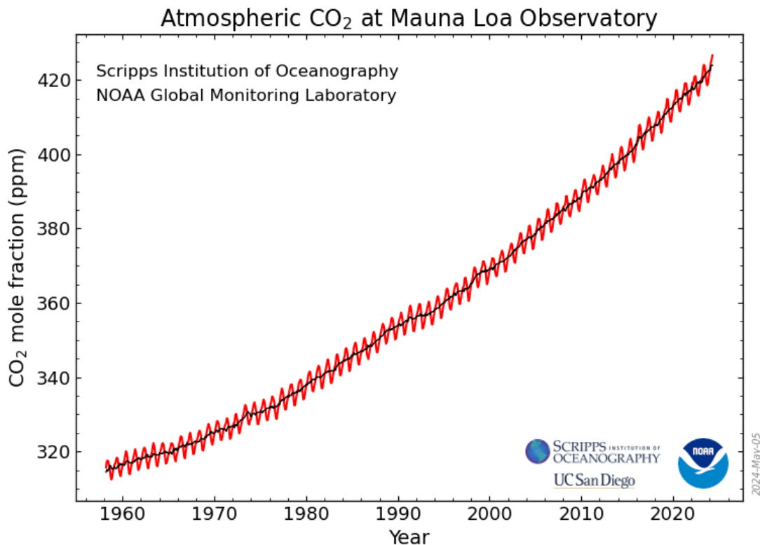
Figure 2. The Keeling Curve: Atmospheric CO 2 Measured at Mauna Loa Observatory
