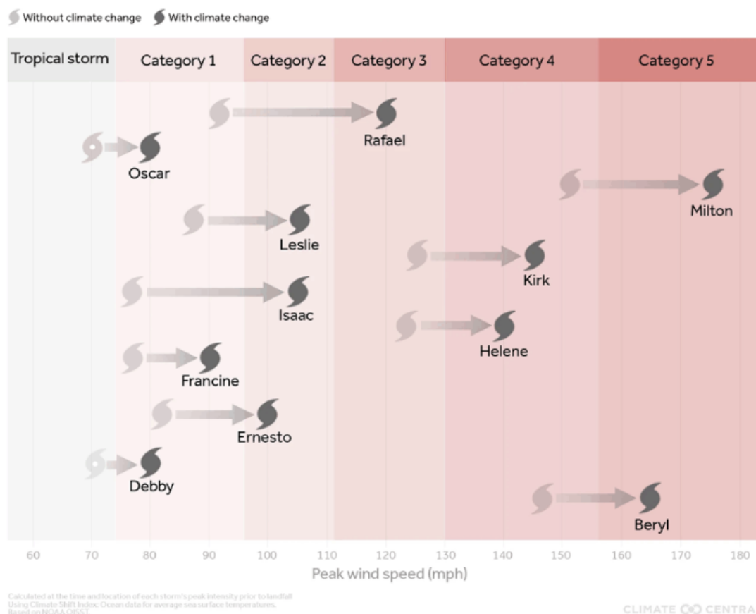
Figure 4. Climate Change Fuels Stronger Storms
