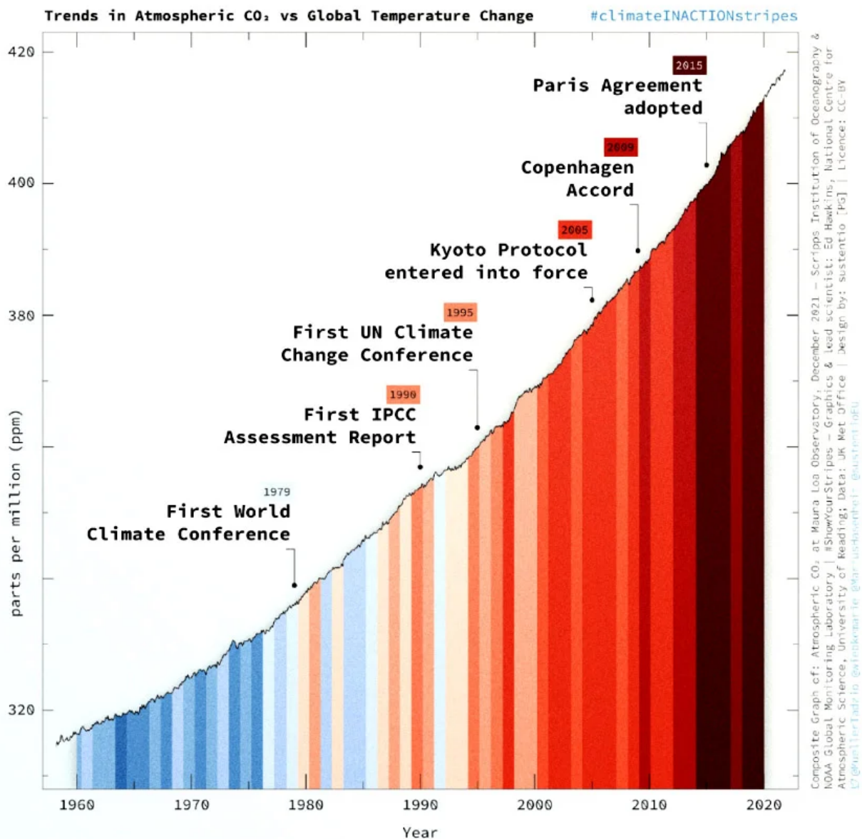
Figure 13. Trends in Atmospheric CO 2 vs Global Temperature Change (From Scientist Rebellion, https://scientistrebellion.org/ )
