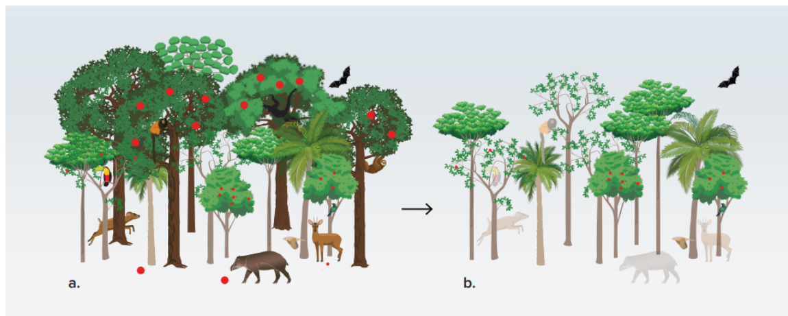
Figure 6. Hunting Can Lead to a Loss of Carbon Storage
